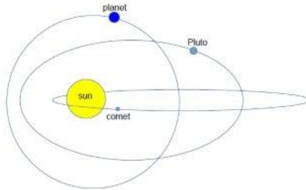
Fig. 4 Formation of planets according to the New Revelation.
