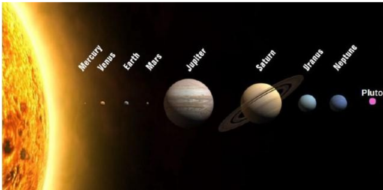
Fig. 5: Planets of the solar system (NASA website).
