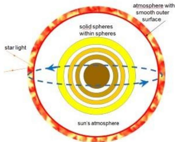
Fig. 6: The structure of the sun according to the New Revelation.
