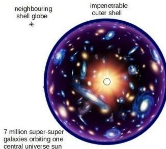
Fig. 3 A Shell-globe according to the New Revelation.
