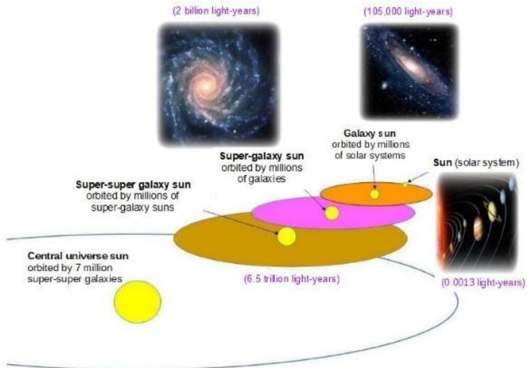
Fig. 2 Structure of the universe as portrayed by the New Revelation.
